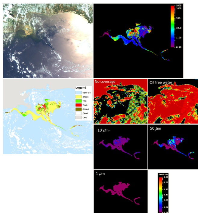
Fig. 31 May 20, 2010, 18:45 GMT. Top left: MODIS RGB image; top right: surface oil volume (liters per MODIS 250-m pixel) (“product I” in Fig. 3); bottom left: surface oil classes (sheen, thin, and thick) (“product I” in Fig. 3); bottom right: surface oil probability (e.g., 0.10 represents that 10% of the surface is covered by the corresponding class) (“product I” in Fig. 3).
