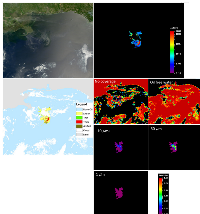
Fig. 28 May 10, 2010, 16:35 GMT. Top left: MODIS RGB image; top right: surface oil volume (liters per MODIS 250-m pixel) (“product I” in Fig. 3); bottom left: surface oil classes (sheen, thin, and thick) (“product I” in Fig. 3); bottom right: surface oil probability (e.g., 0.10 represents that 10% of the surface is covered by the corresponding class) (“product I” in Fig. 3).
