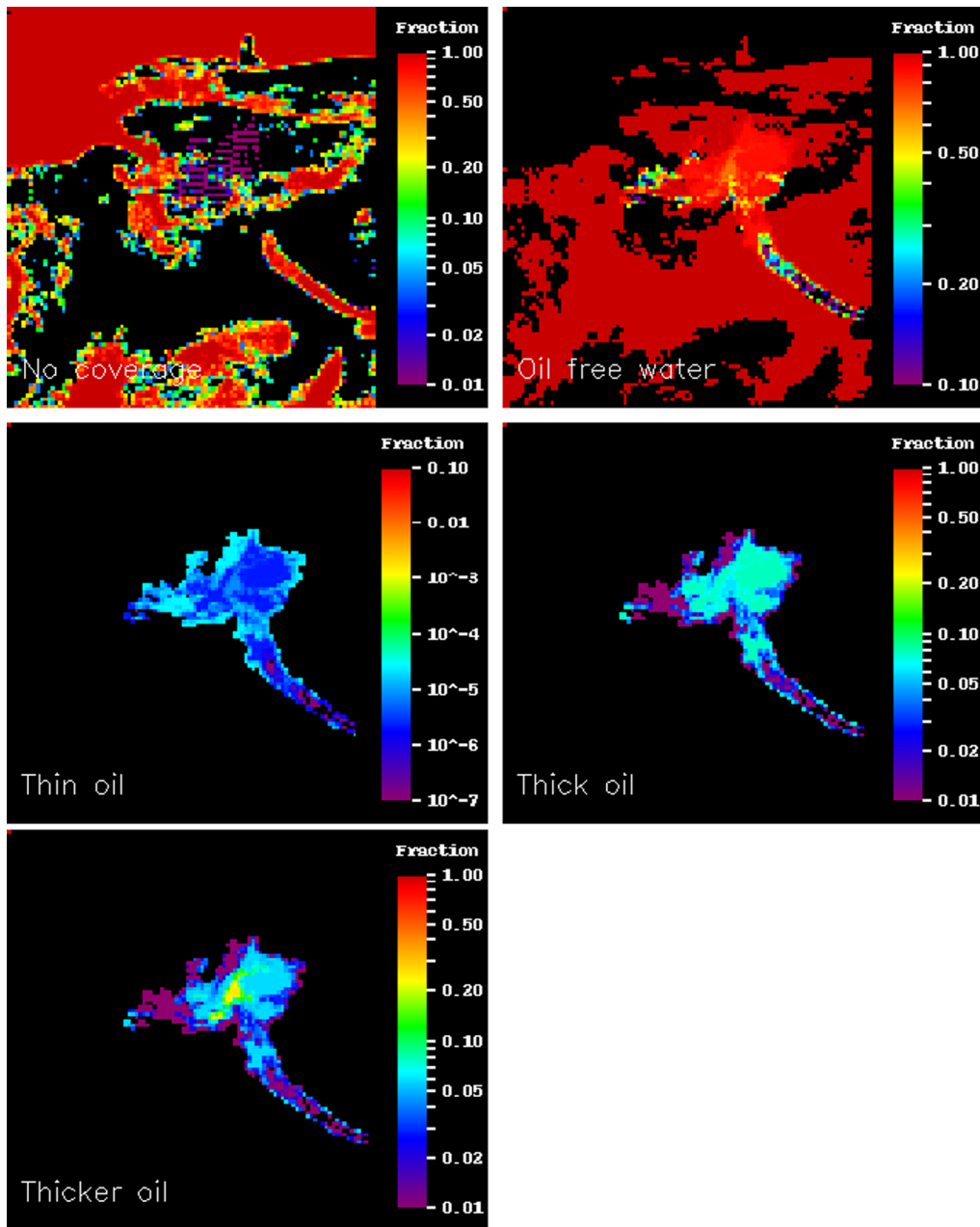
Fig. 13 An example of MODIS oil probability distribution maps for May 17, 2010 (same as in Fig. 12). These maps are listed as “product III” in Fig. 3. The different classes are defined in Table 2: thin: <1.7 \mu\text{m} (mean = 1 \mu\text{m} ); thick: 1.7 to 20 \mu\text{m} (mean = 10 \mu\text{m} ); thicker: >20 \mu\text{m} (mean = 50 \mu\text{m} ). For each 5-km grid cell, the sum probability for all five classes (no observation, oil-free water, thin, thick, and thicker oil) adds up to 1.0. A value of 0.20 in a certain grid cell in the thicker oil class means that 20% of that cell contains thicker oil. Note that because of the large pixel size, most of the pixel is not covered by any oil (i.e., large fractional values in the oil-free water map).
