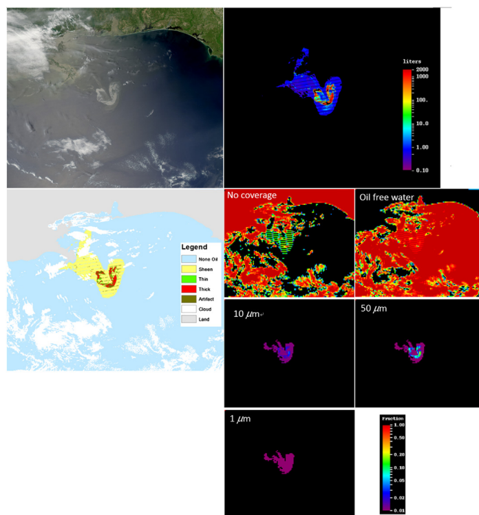
Fig. 27 September 05, 2010, 19:05 GMT. Top left: MODIS RGB image; top right: surface oil volume (liters per MODIS 250-m pixel) (“product I” in Fig. 3); bottom left: surface oil classes (sheen, thin, and thick) (“Product I” in Fig. 3); bottom right: surface oil probability (e.g., 0.10 represents that 10% of the surface is covered by the corresponding class) (“product I” in Fig. 3).
